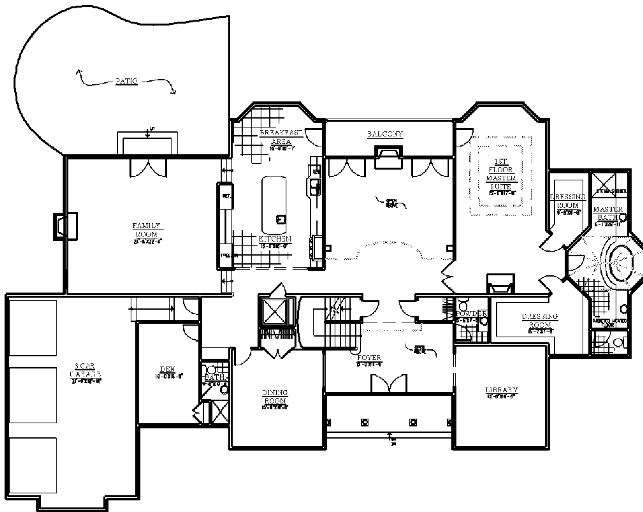
FIRST FLOOR PLAN 12'-0" x 11'-4"
